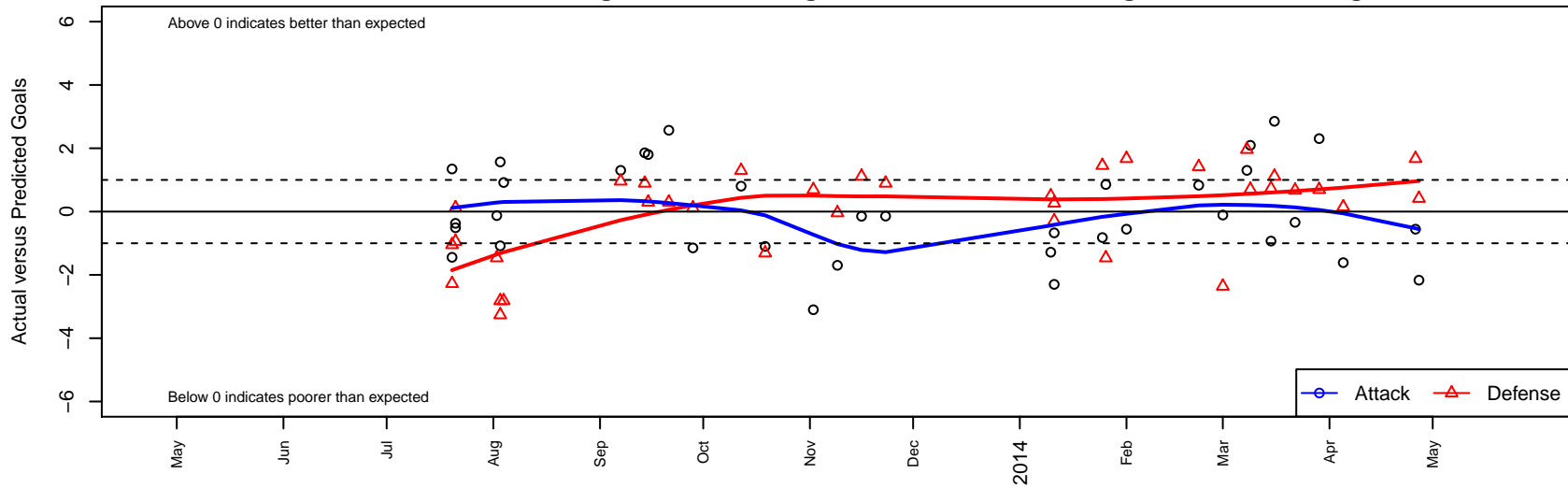
Blackhills FC Black G02 Dots are actual minus expected GF (blue circles) and GA (red triangles). Blue line is smoothed change in attack strength. Red is smoothed change in defense strength.
